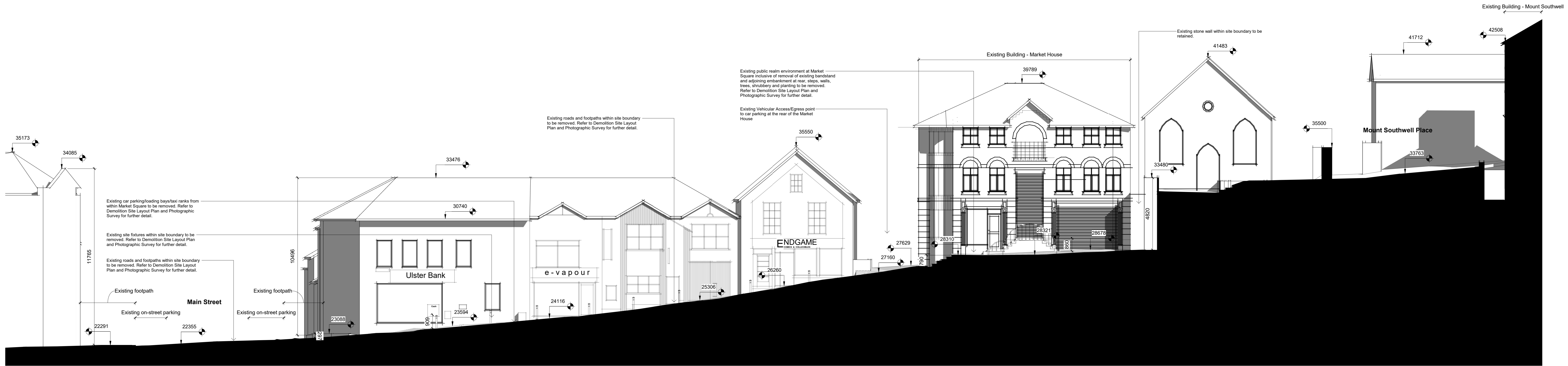
Existing Sectional Elevation 03 1 : 100
